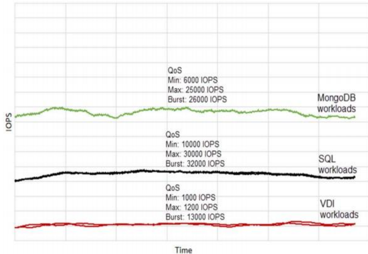
Mixed workloads with QoS
