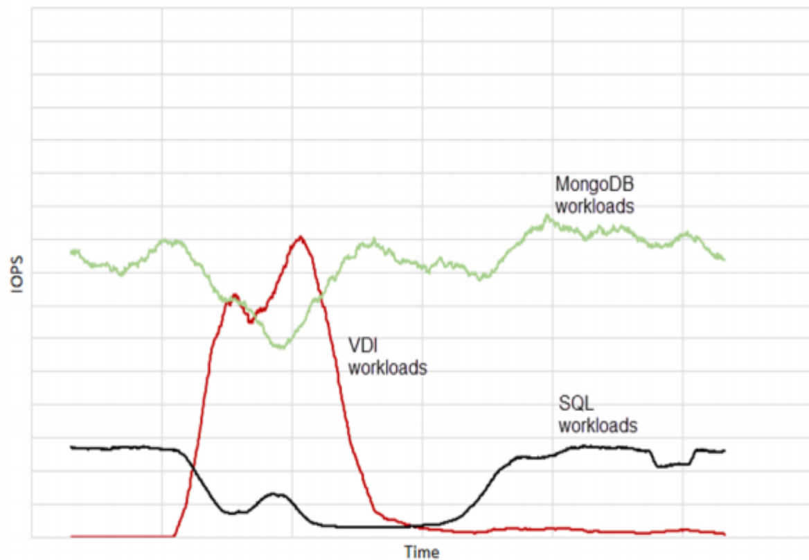
Mixed workloads without QoS type control
